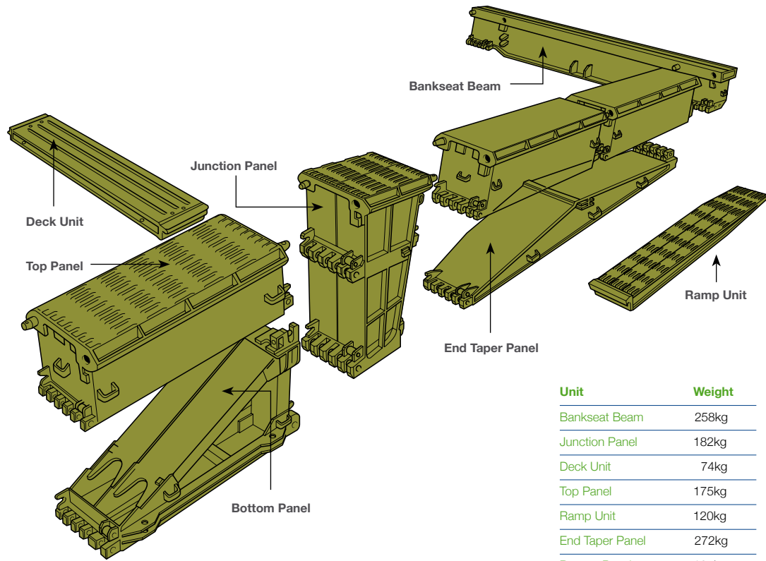
Single Storey bridge configuration
